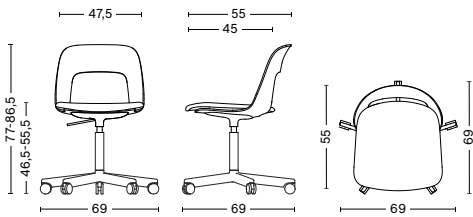
LAYOUT CHAIR 143 Width 69 cm Depth 69 cm Height 77-86,5 cm Seat height 46,5-55,5 cm Weight 9,8 kg
