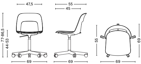
LAYOUT CHAIR 141 Width 69 cm Depth 69 cm Height 77-86,5 cm Seat height 44-53 cm Weight 9,5 kg
