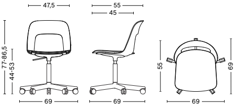
LAYOUT CHAIR 142 Width 69 cm Depth 69 cm Height 77-86,5 cm Seat height 44-53 cm Weight 9,3 kg
