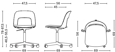
LAYOUT CHAIR 144 Width 69 cm Depth 69 cm Height 78-87,5 cm Seat height 46,5-55,5 cm Weight 10,2 kg
